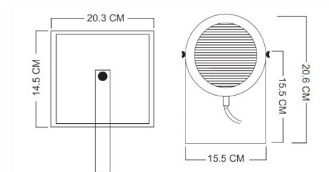
Mounting Detail
